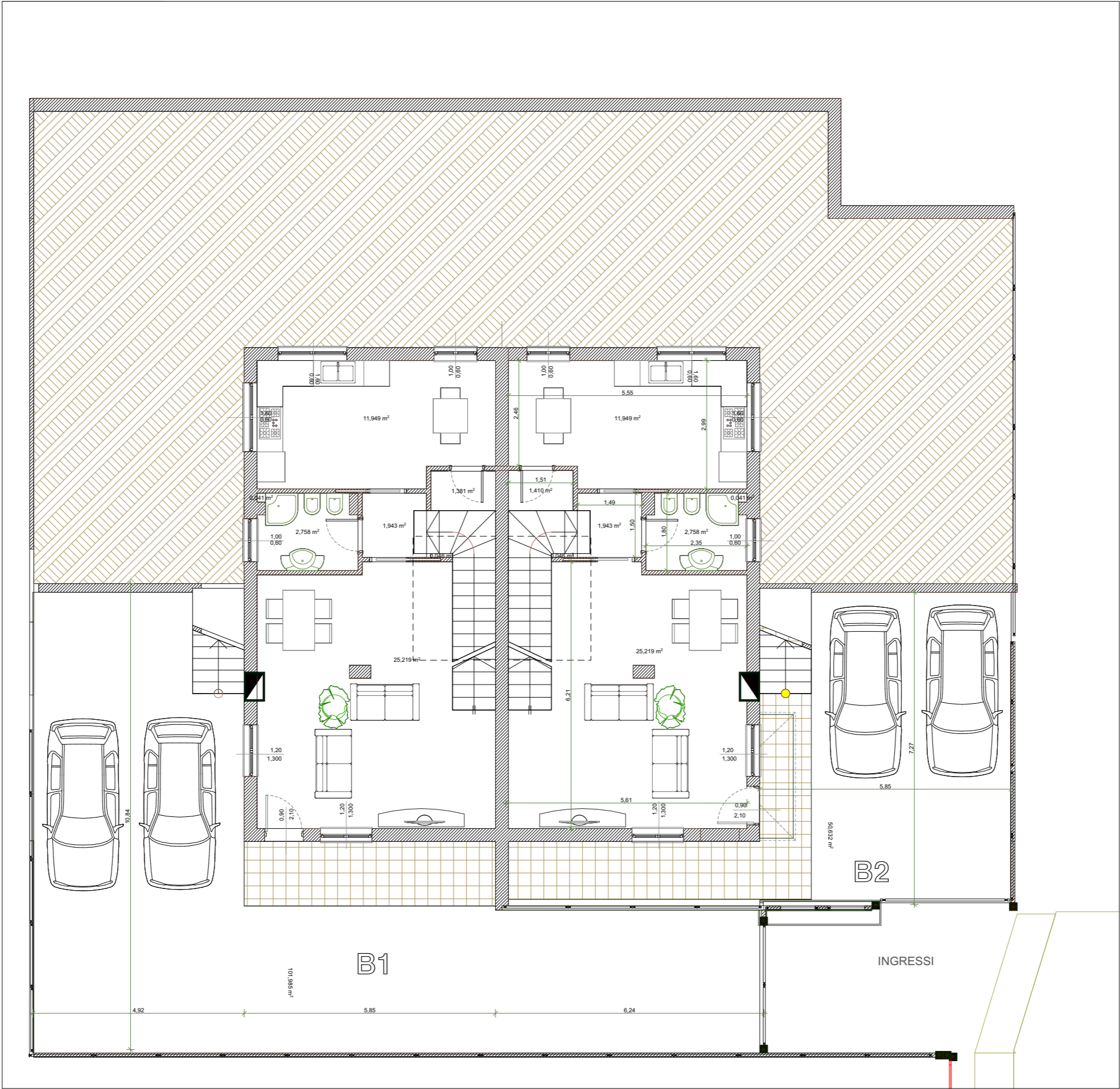
PIANO TERRA SCALA 1:100
